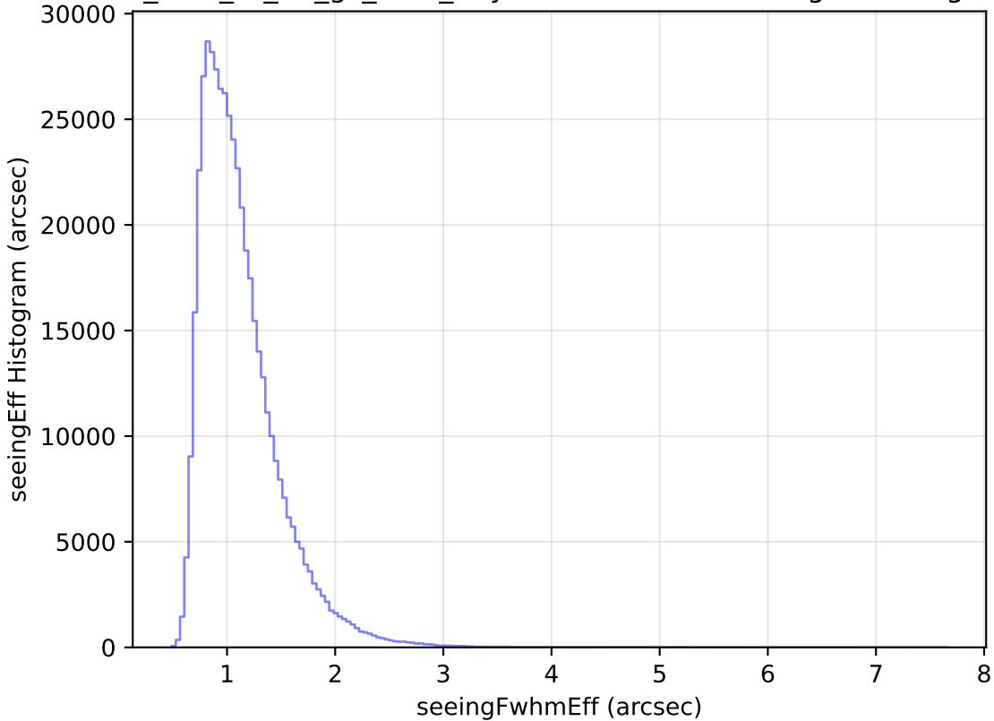
too_elab_r8_d3_gz_v3.4_10yrs WFD r band: seeingEff Histogram
