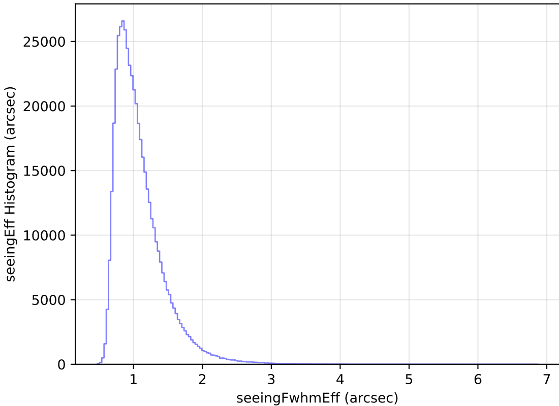
too_elab_r8_d3_gz_v3.4_10yrs WFD i band: seeingEff Histogram
