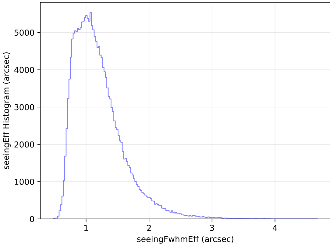
too_elab_r8_d3_gz_v3.4_10yrs WFD g band: seeingEff Histogram
