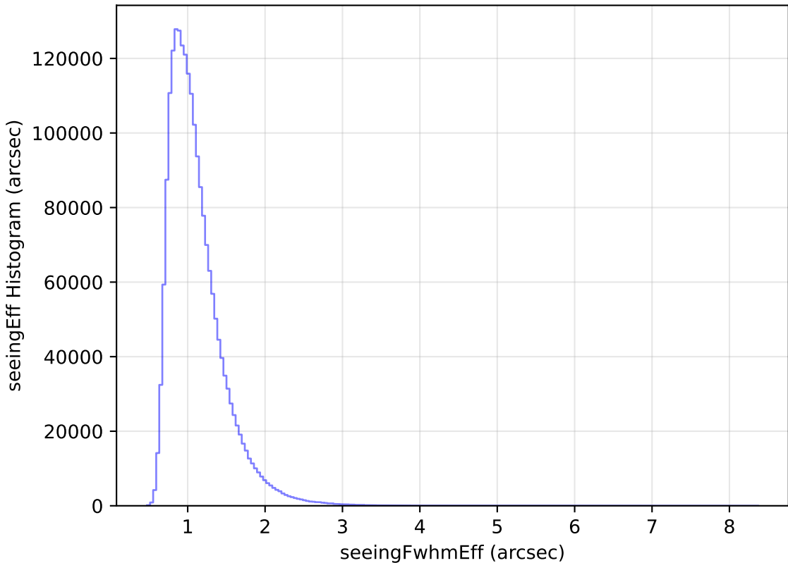
too_elab_r8_d3_gz_v3.4_10yrs WFD all bands: seeingEff Histogram
