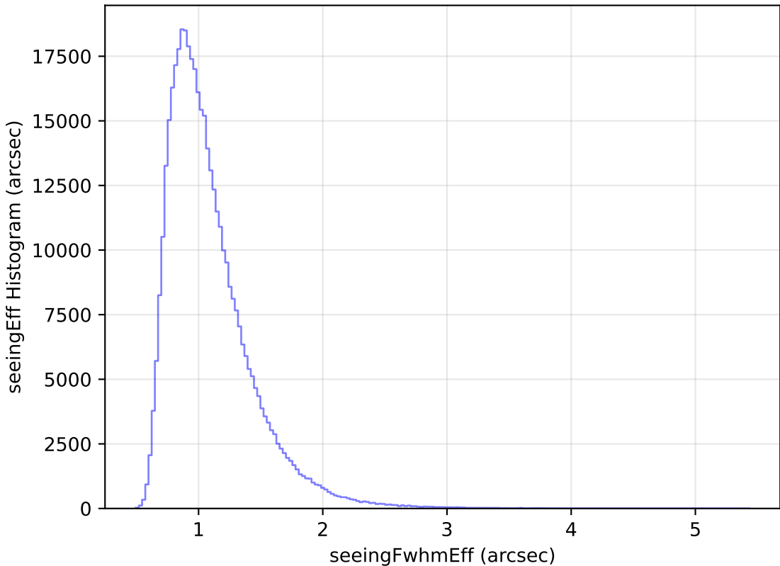
too_elab_r8_d3_gz_v3.4_10yrs All sky z band: seeingEff Histogram
