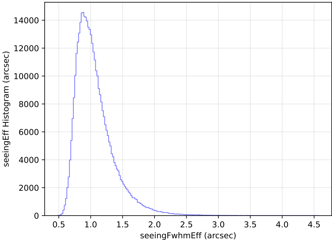
too_elab_r8_d3_gz_v3.4_10yrs All sky y band: seeingEff Histogram
