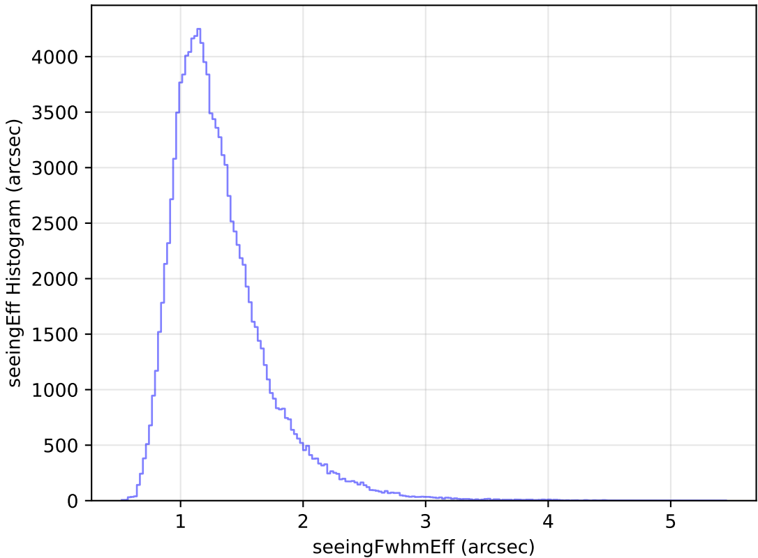
too_elab_r8_d3_gz_v3.4_10yrs All sky u band: seeingEff Histogram
