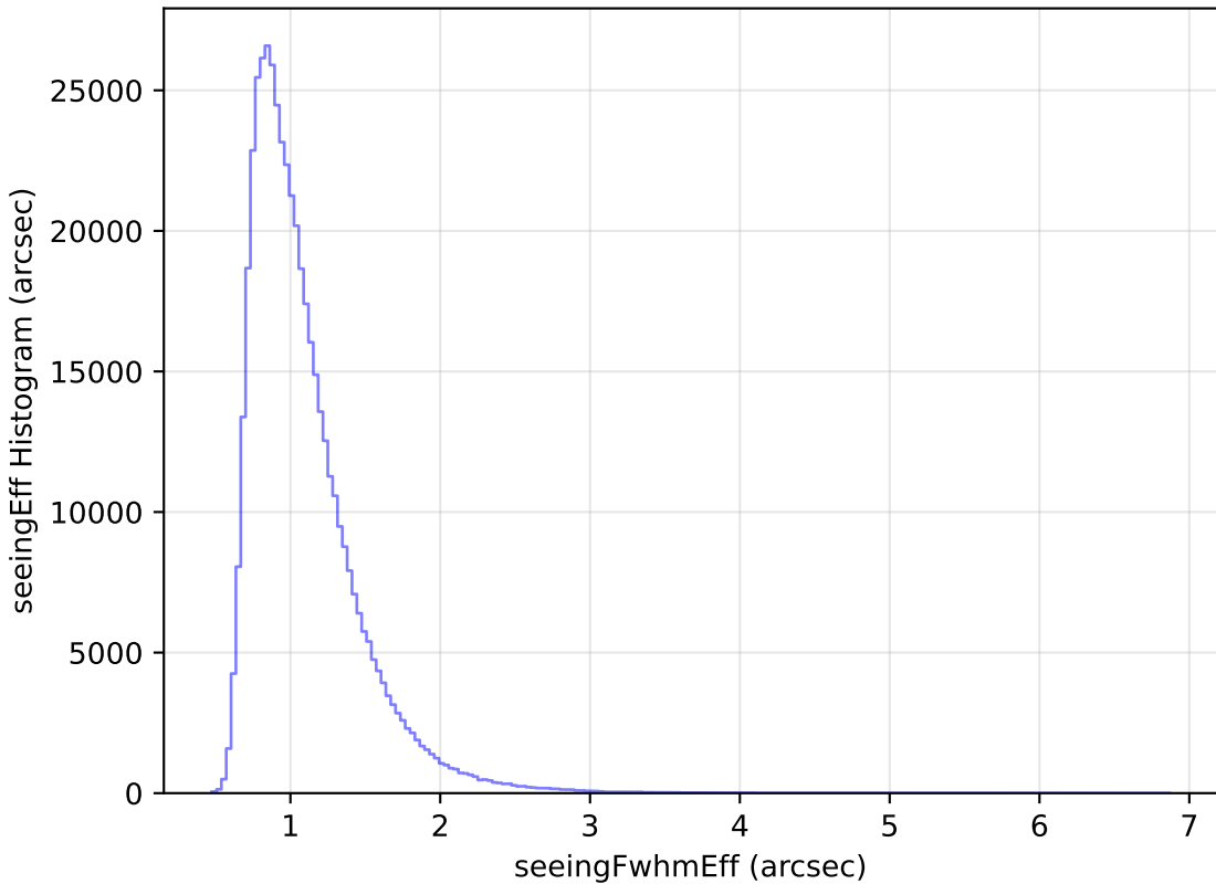
too_elab_r8_d3_gz_v3.4_10yrs All sky i band: seeingEff Histogram
