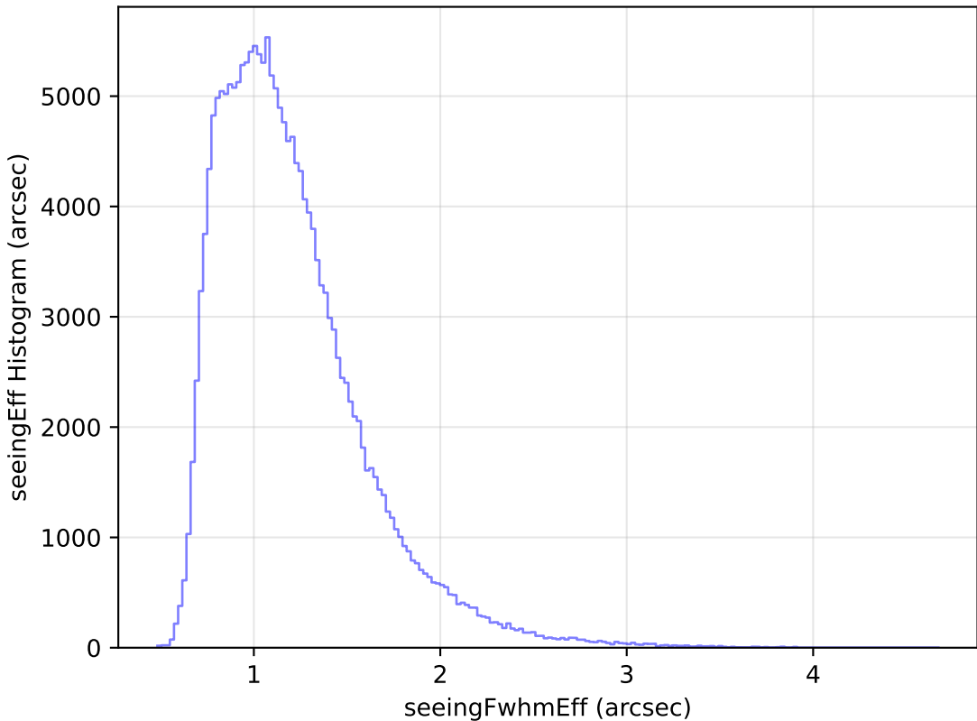
too_elab_r8_d3_gz_v3.4_10yrs All sky g band: seeingEff Histogram
