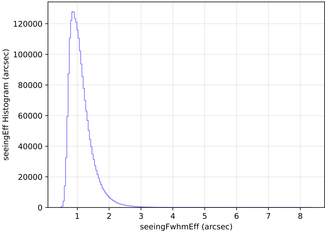
too_elab_r8_d3_gz_v3.4_10yrs All sky all bands: seeingEff Histogram
