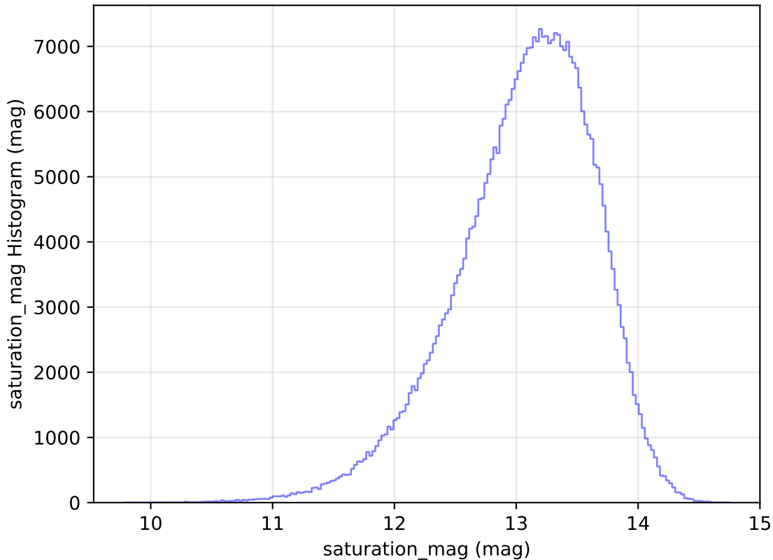
too_elab_r8_d3_gz_v3.4_10yrs WFD y band: saturation_mag Histogram
