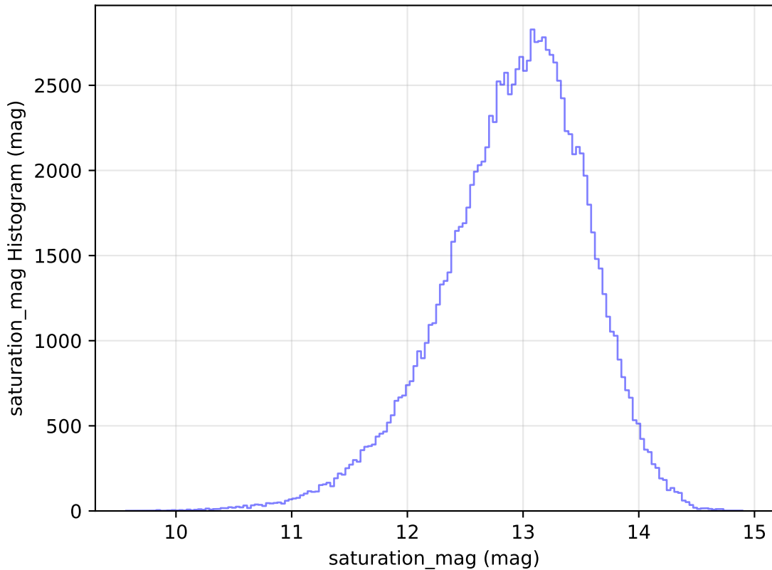
too_elab_r8_d3_gz_v3.4_10yrs WFD u band: saturation_mag Histogram
