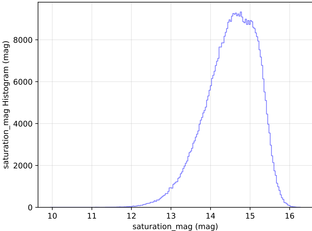
too_elab_r8_d3_gz_v3.4_10yrs WFD r band: saturation_mag Histogram
