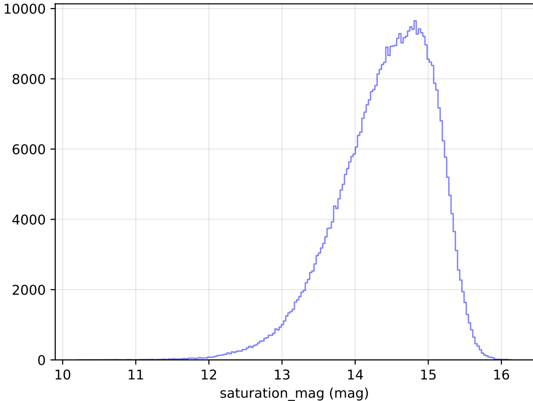
too_elab_r8_d3_gz_v3.4_10yrs WFD i band: saturation_mag Histogram
