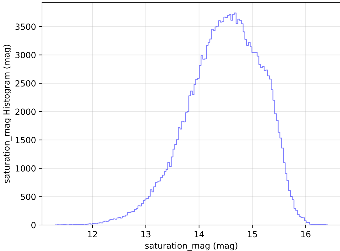
too_elab_r8_d3_gz_v3.4_10yrs WFD g band: saturation_mag Histogram
