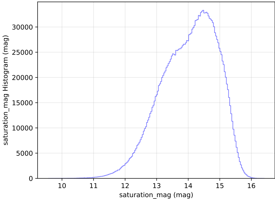
too_elab_r8_d3_gz_v3.4_10yrs WFD all bands: saturation_mag Histogram
