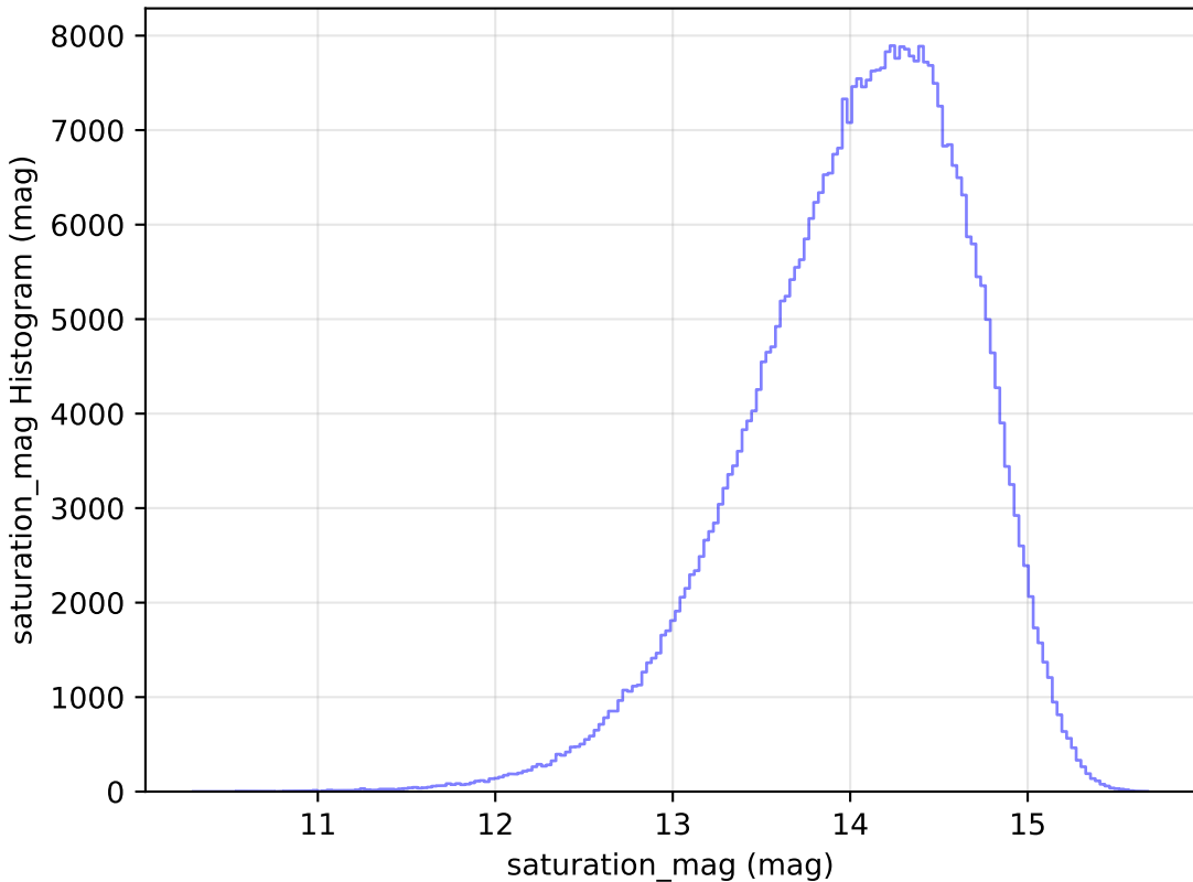
too_elab_r8_d3_gz_v3.4_10yrs All sky z band: saturation_mag Histogram
