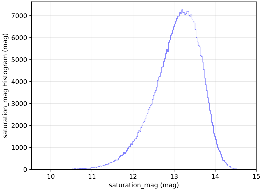
too_elab_r8_d3_gz_v3.4_10yrs All sky y band: saturation_mag Histogram
