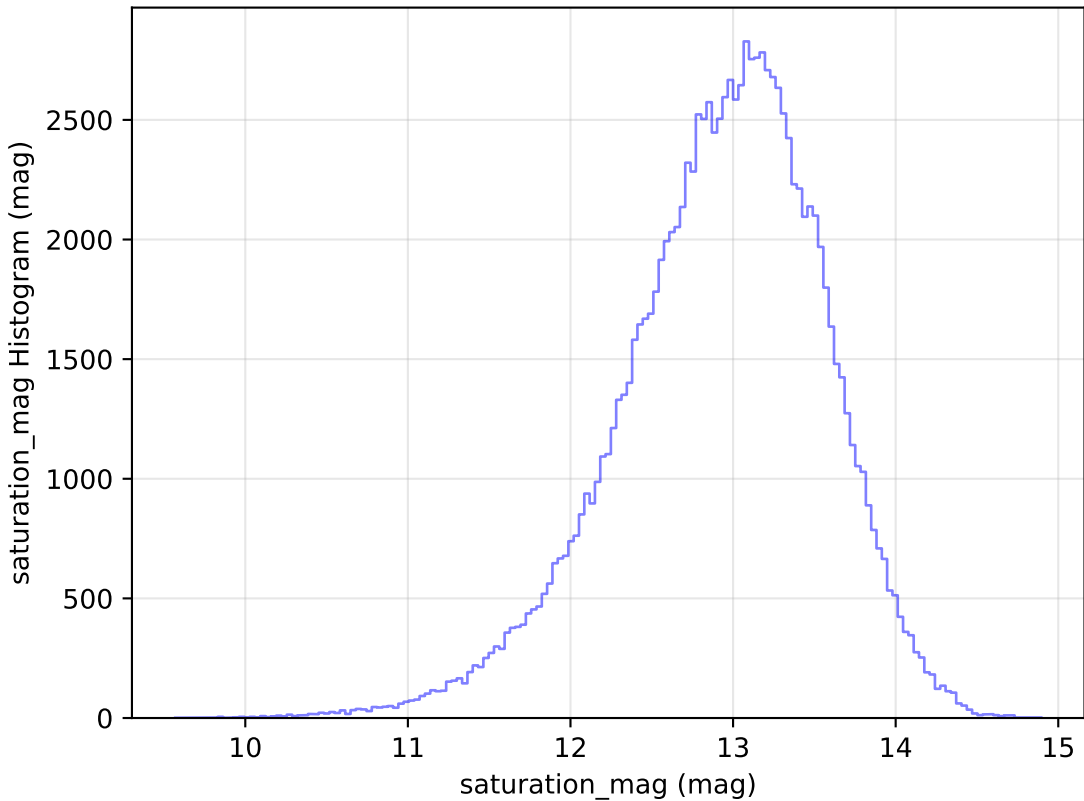
too_elab_r8_d3_gz_v3.4_10yrs All sky u band: saturation_mag Histogram
