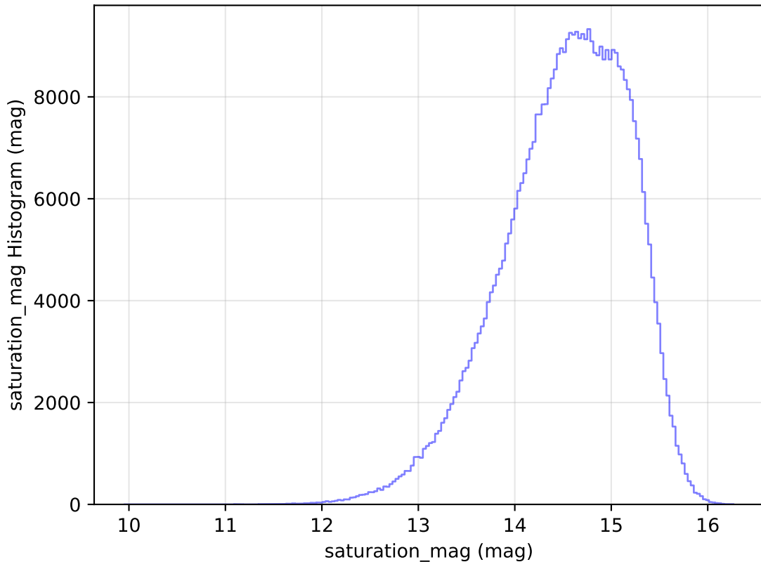
too_elab_r8_d3_gz_v3.4_10yrs All sky r band: saturation_mag Histogram
