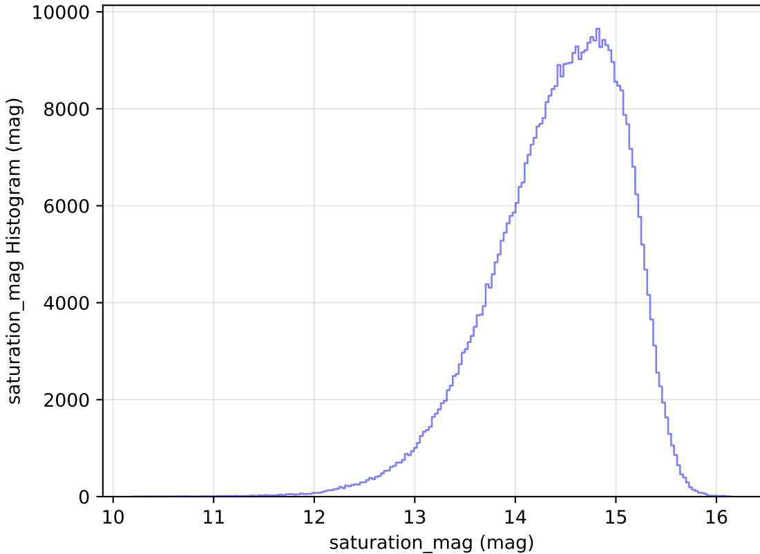
too_elab_r8_d3_gz_v3.4_10yrs All sky i band: saturation_mag Histogram
