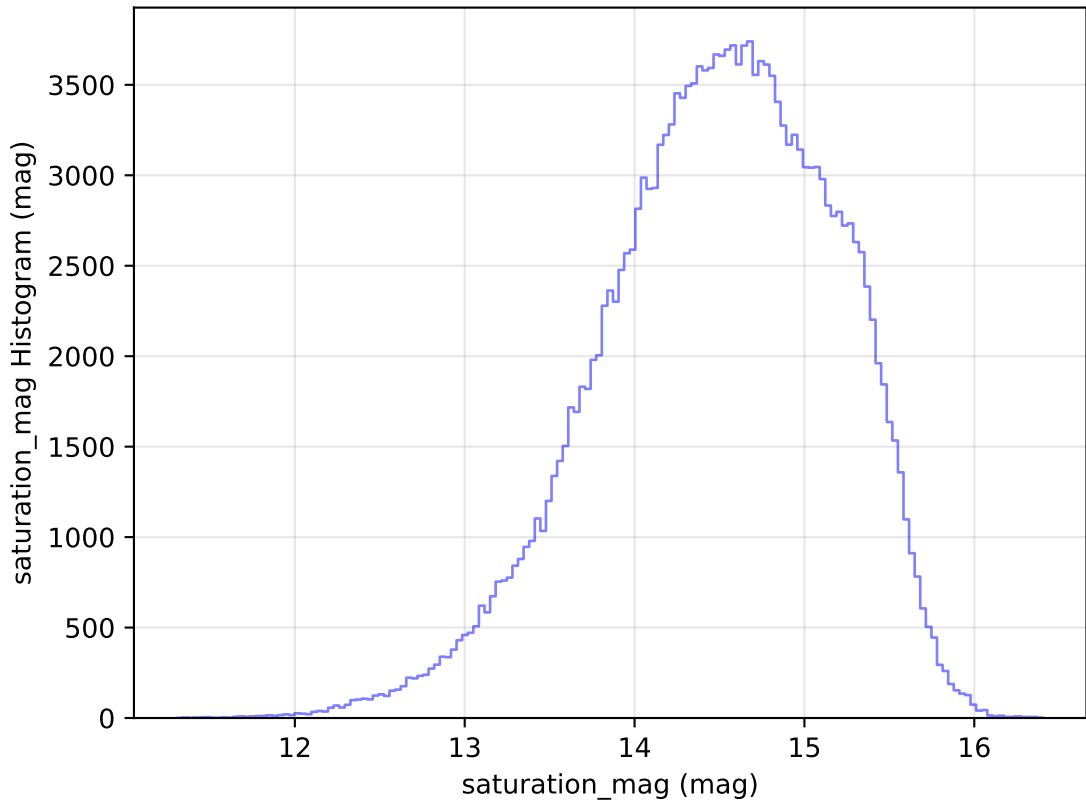
too_elab_r8_d3_gz_v3.4_10yrs All sky g band: saturation_mag Histogram
