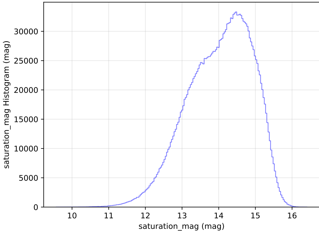
too_elab_r8_d3_gz_v3.4_10yrs All sky all bands: saturation_mag Histogram
