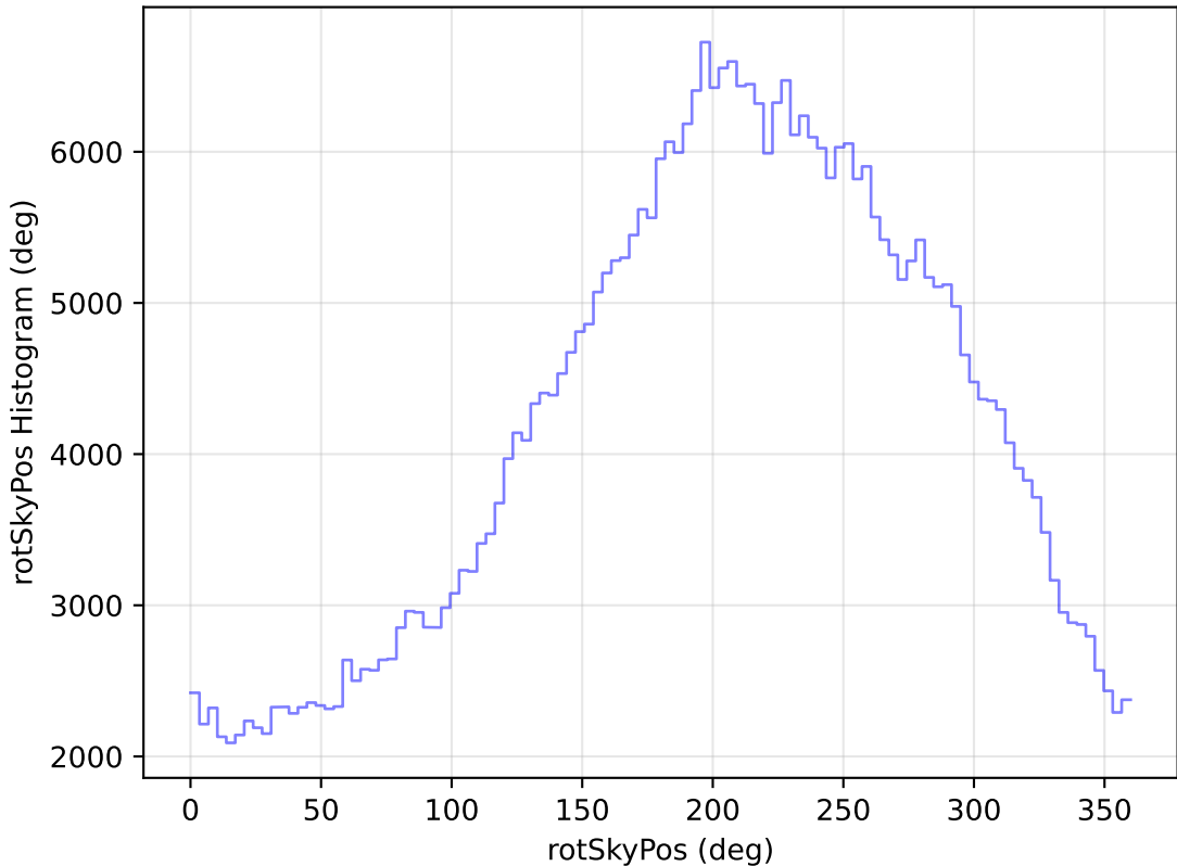
too_elab_r8_d3_gz_v3.4_10yrs WFD z band: rotSkyPos Histogram
