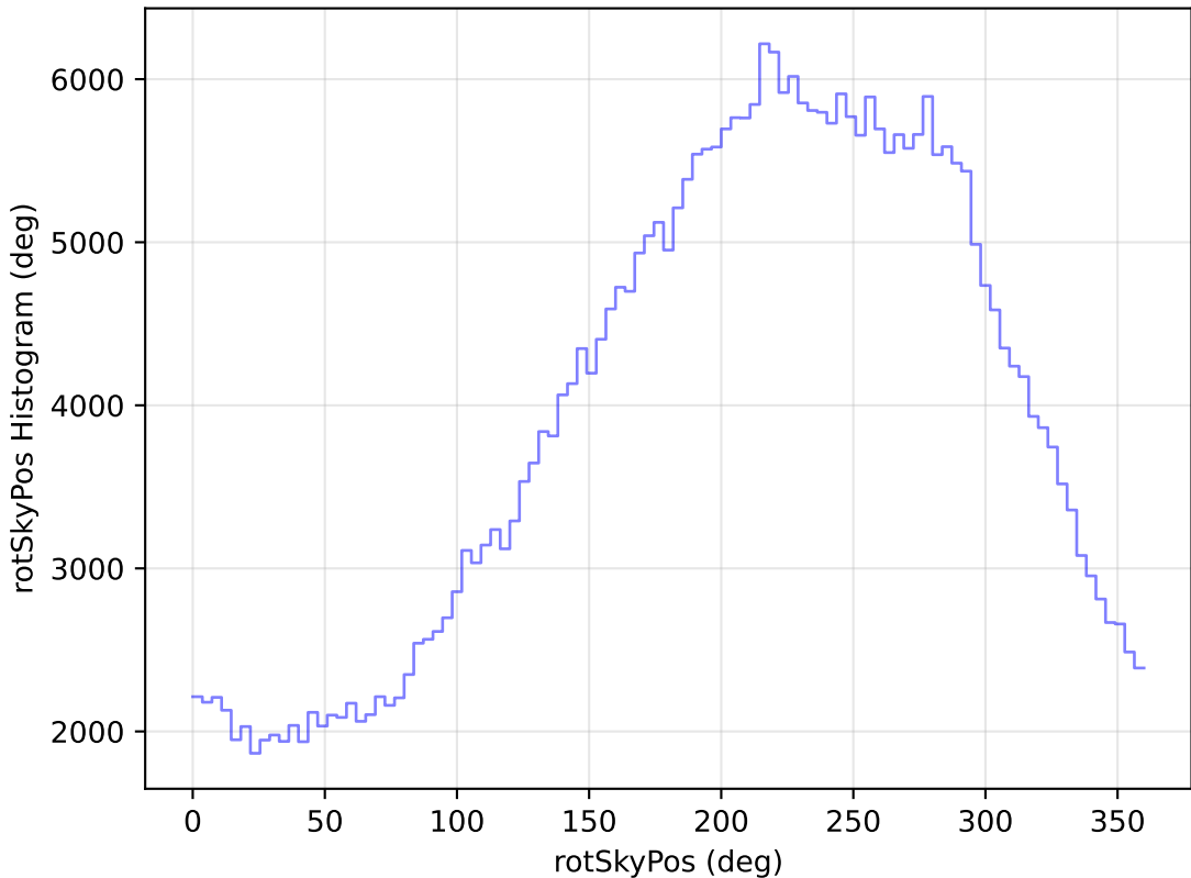
too_elab_r8_d3_gz_v3.4_10yrs WFD y band: rotSkyPos Histogram
