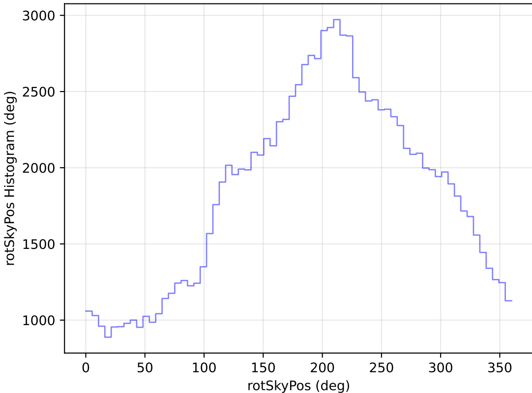
too_elab_r8_d3_gz_v3.4_10yrs WFD u band: rotSkyPos Histogram
