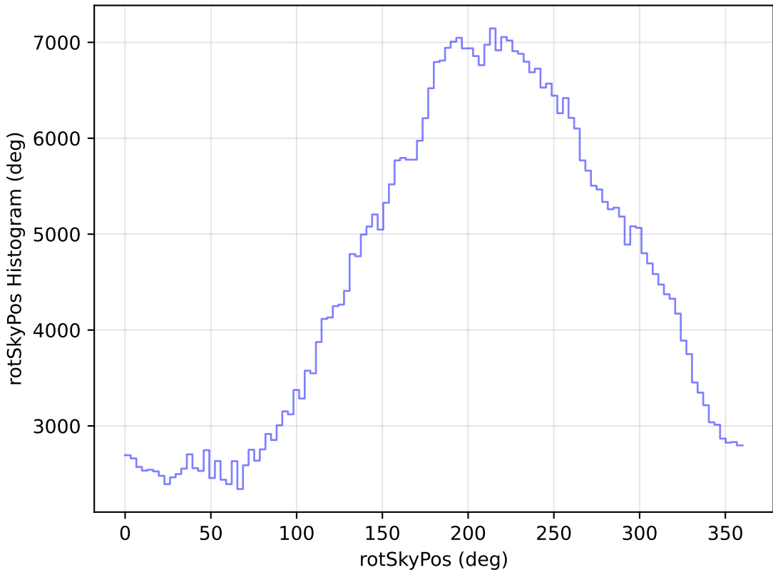
too_elab_r8_d3_gz_v3.4_10yrs WFD i band: rotSkyPos Histogram
