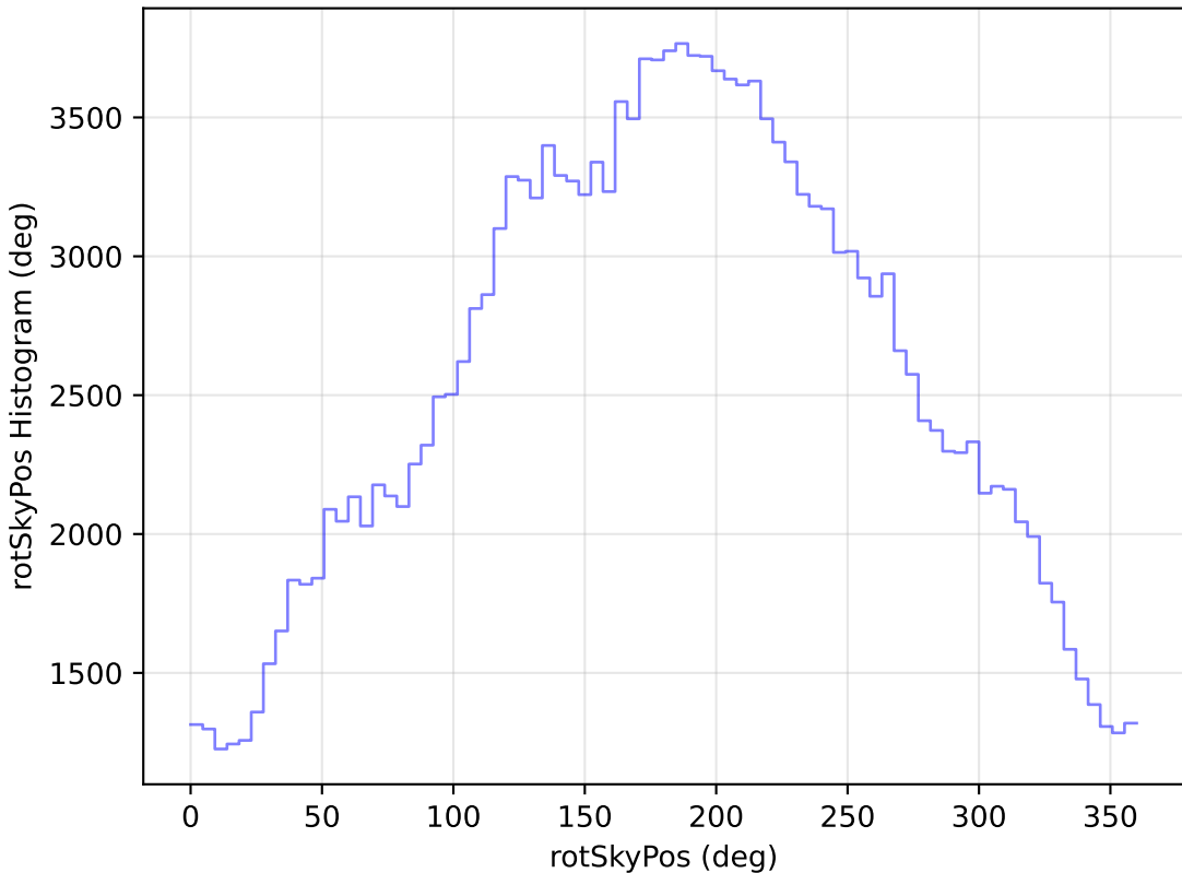
too_elab_r8_d3_gz_v3.4_10yrs WFD g band: rotSkyPos Histogram
