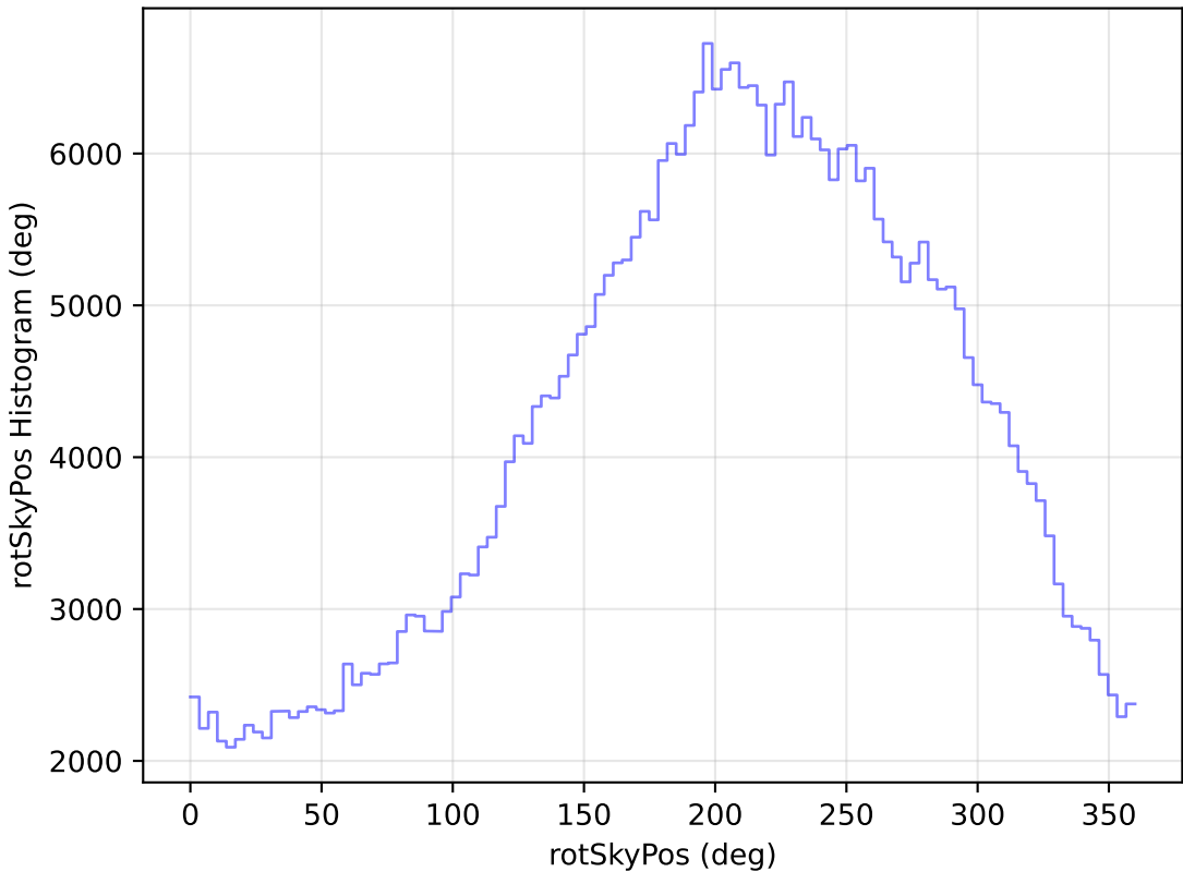
too_elab_r8_d3_gz_v3.4_10yrs All sky z band: rotSkyPos Histogram
