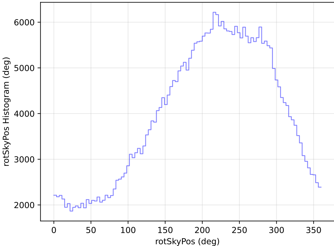
too_elab_r8_d3_gz_v3.4_10yrs All sky y band: rotSkyPos Histogram
