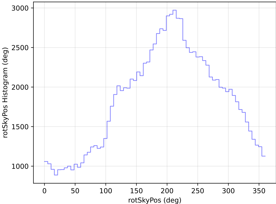
too_elab_r8_d3_gz_v3.4_10yrs All sky u band: rotSkyPos Histogram
