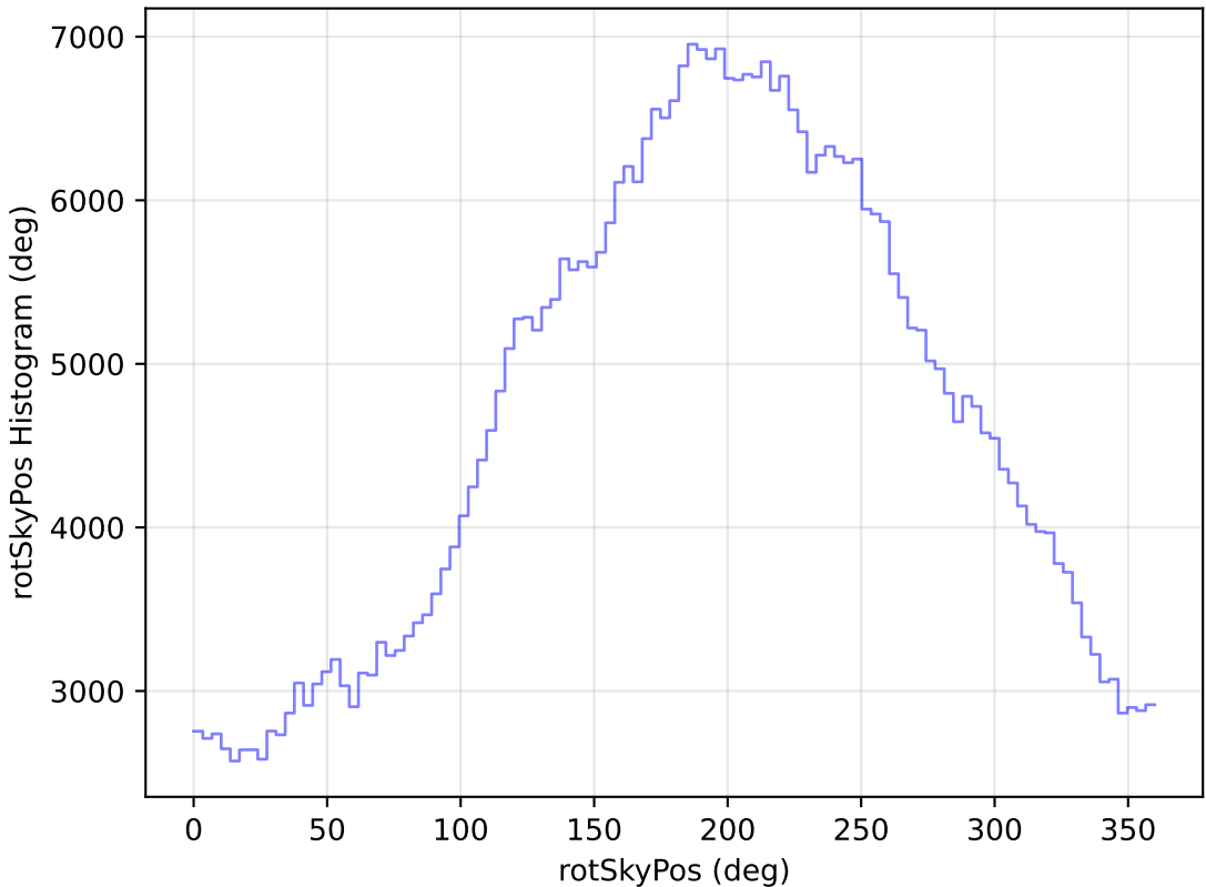
too_elab_r8_d3_gz_v3.4_10yrs All sky r band: rotSkyPos Histogram
