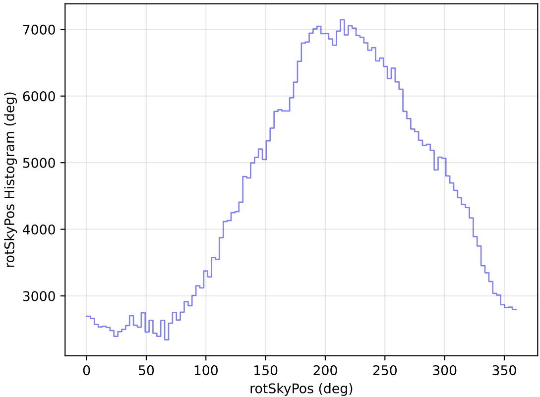
too_elab_r8_d3_gz_v3.4_10yrs All sky i band: rotSkyPos Histogram
