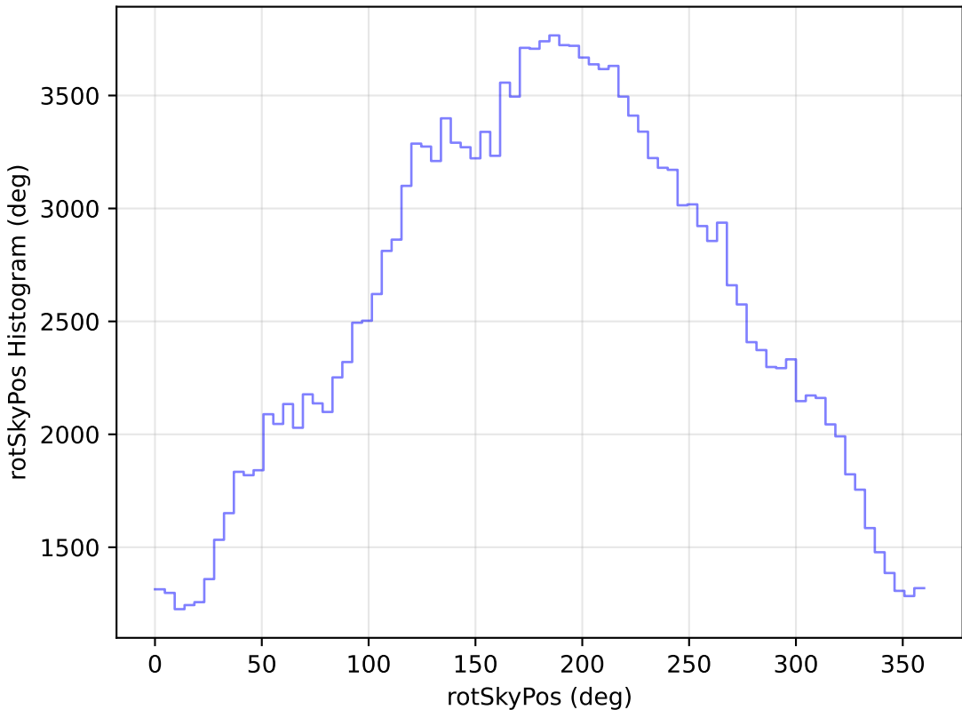
too_elab_r8_d3_gz_v3.4_10yrs All sky g band: rotSkyPos Histogram
