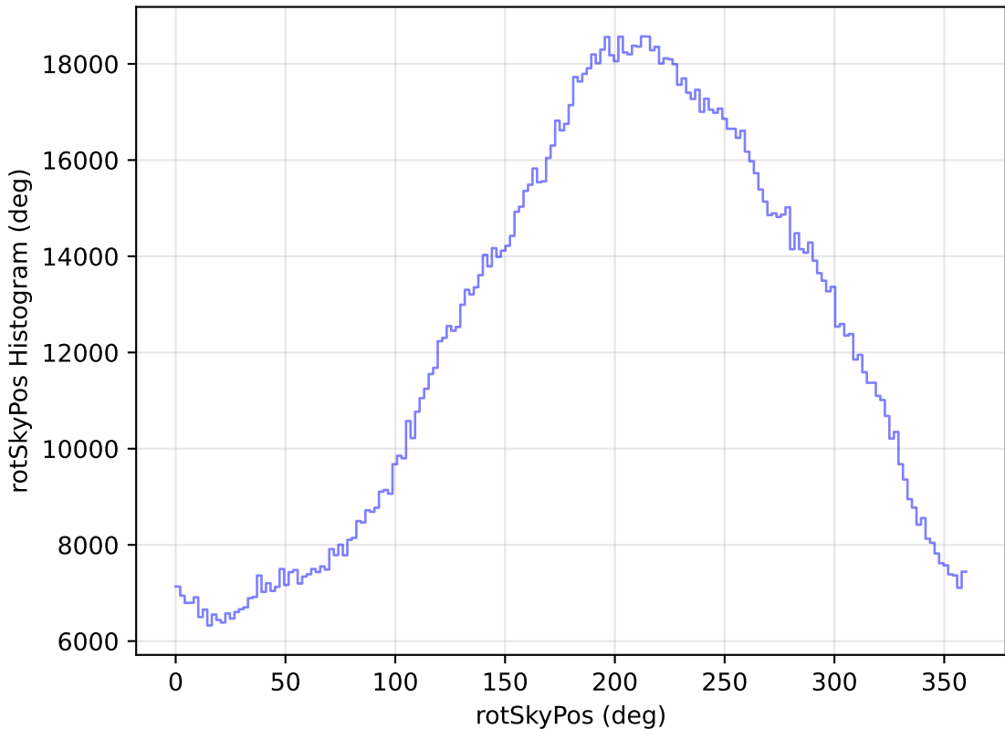
too_elab_r8_d3_gz_v3.4_10yrs All sky all bands: rotSkyPos Histogram
