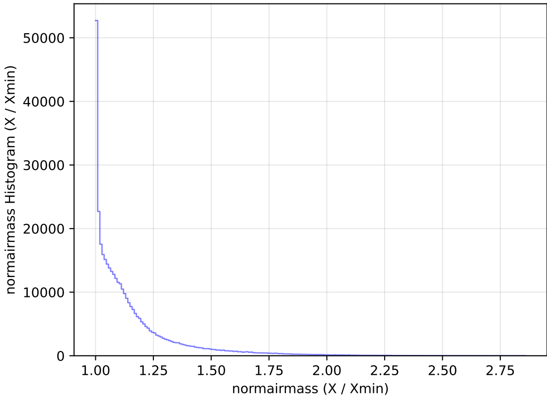
too_elab_r8_d3_gz_v3.4_10yrs WFD y band: normairmass Histogram
