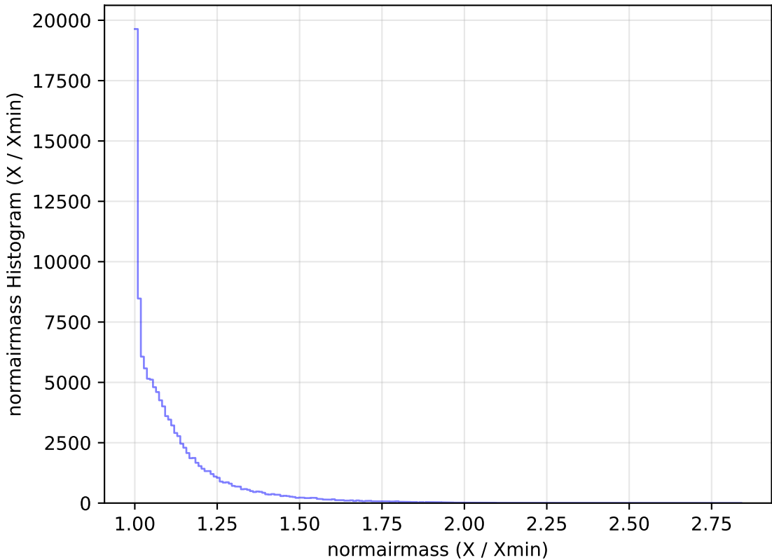
too_elab_r8_d3_gz_v3.4_10yrs WFD u band: normairmass Histogram
