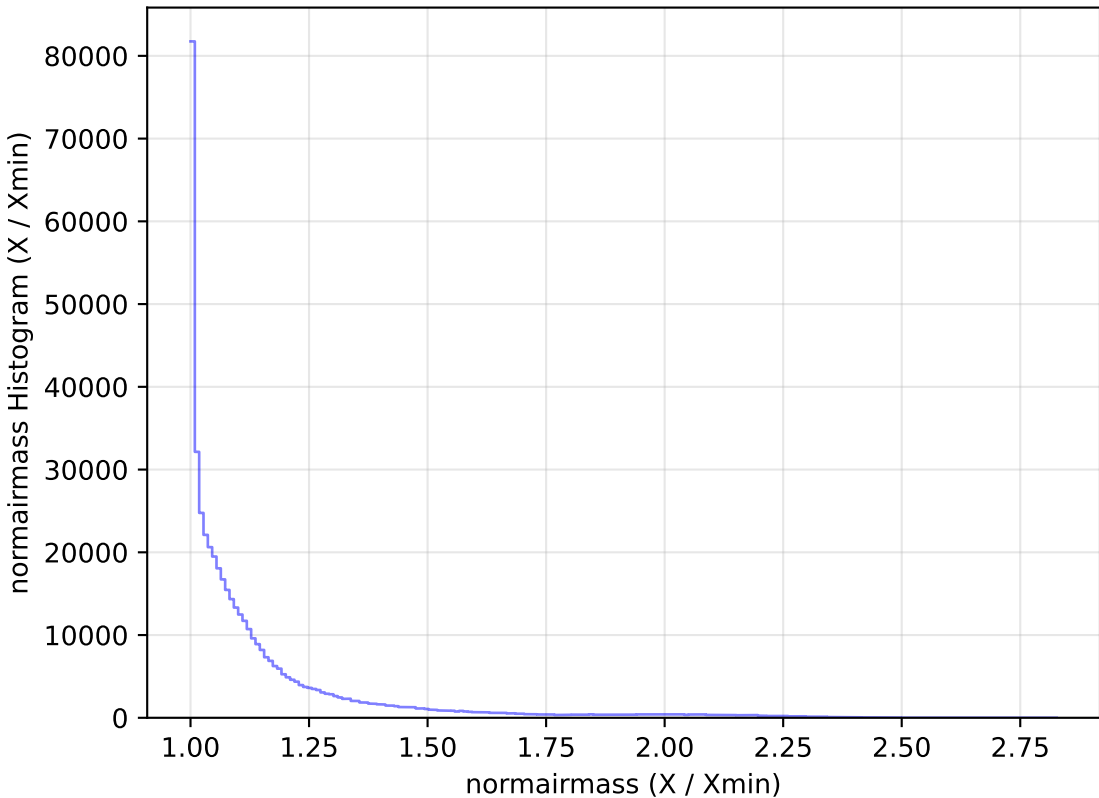
too_elab_r8_d3_gz_v3.4_10yrs WFD r band: normairmass Histogram
