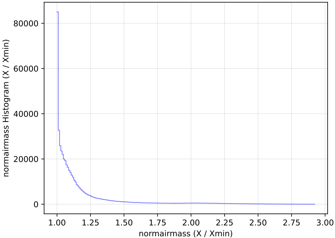
too_elab_r8_d3_gz_v3.4_10yrs WFD i band: normairmass Histogram
