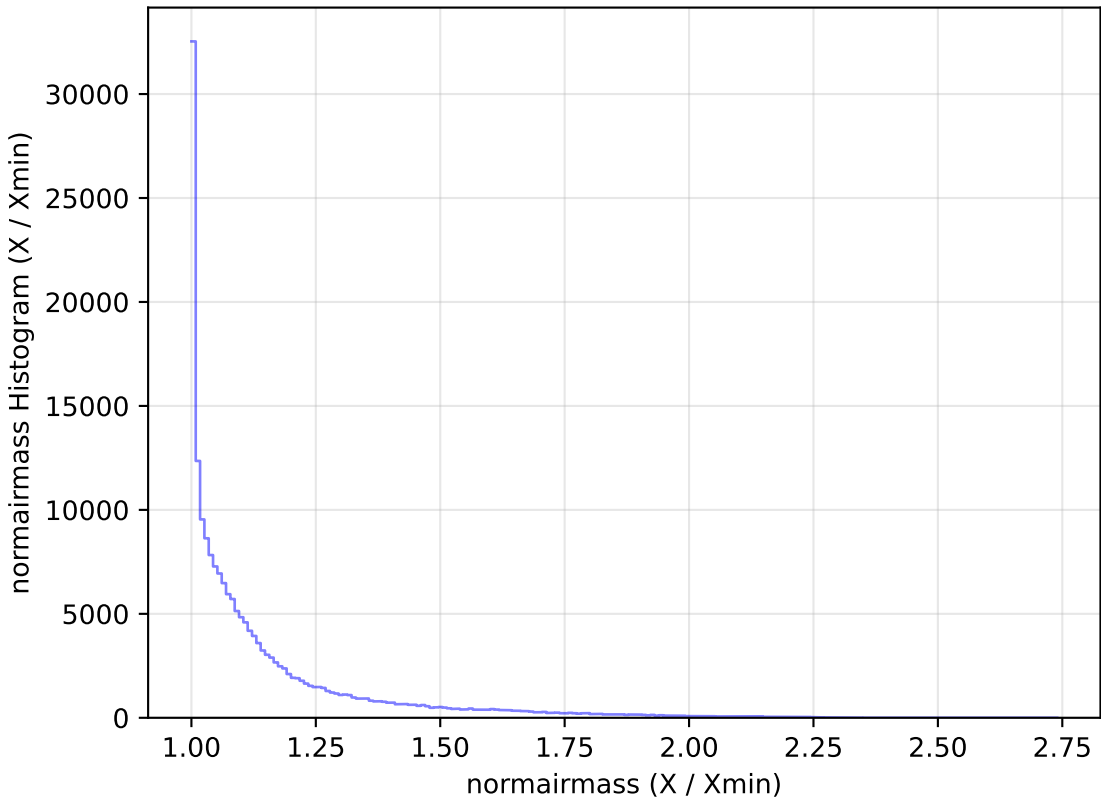
too_elab_r8_d3_gz_v3.4_10yrs WFD g band: normairmass Histogram
