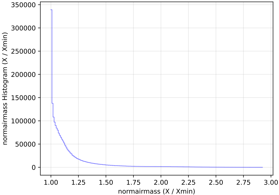
too_elab_r8_d3_gz_v3.4_10yrs WFD all bands: normairmass Histogram
