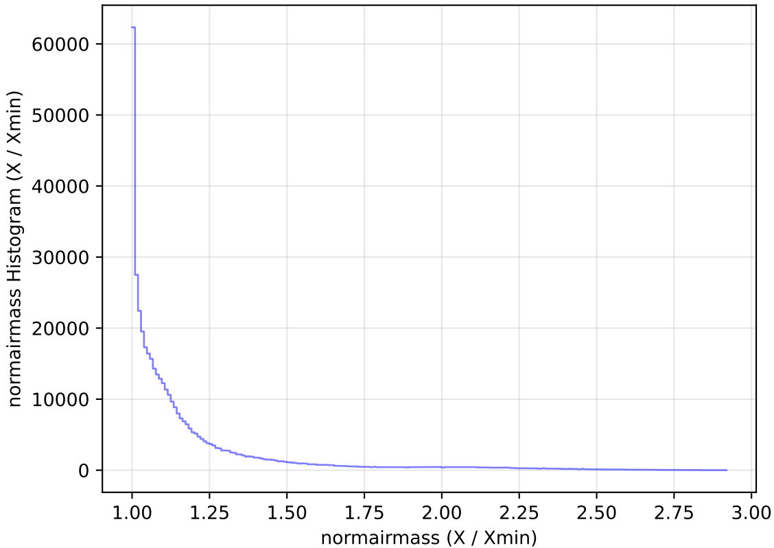
too_elab_r8_d3_gz_v3.4_10yrs All sky z band: normairmass Histogram
