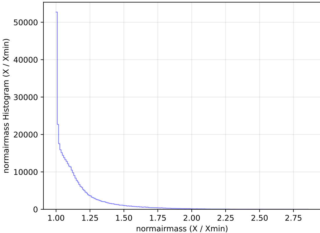
too_elab_r8_d3_gz_v3.4_10yrs All sky y band: normairmass Histogram
