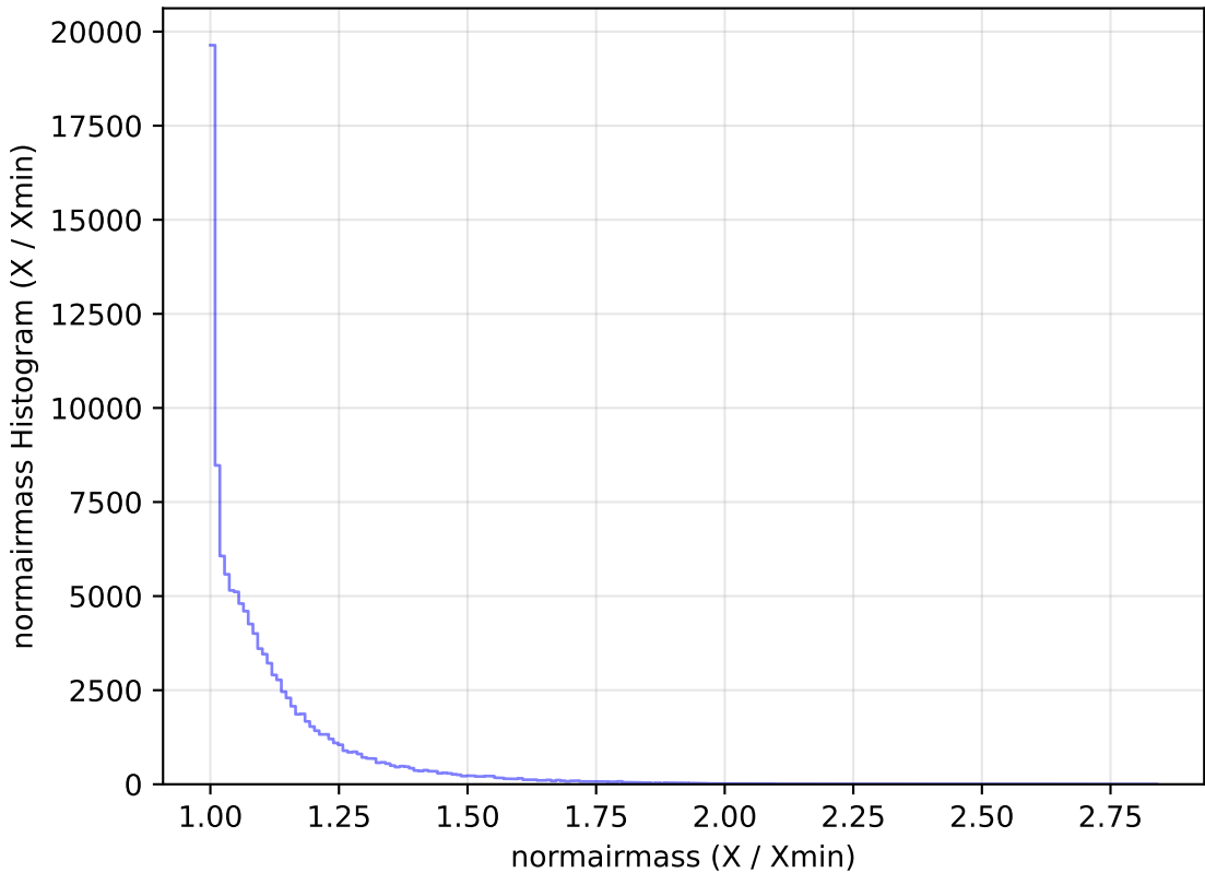
too_elab_r8_d3_gz_v3.4_10yrs All sky u band: normairmass Histogram
