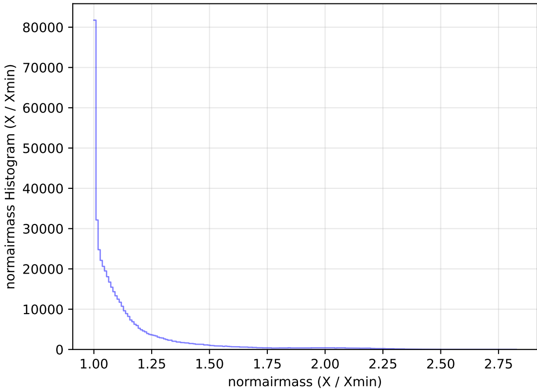
too_elab_r8_d3_gz_v3.4_10yrs All sky r band: normairmass Histogram
