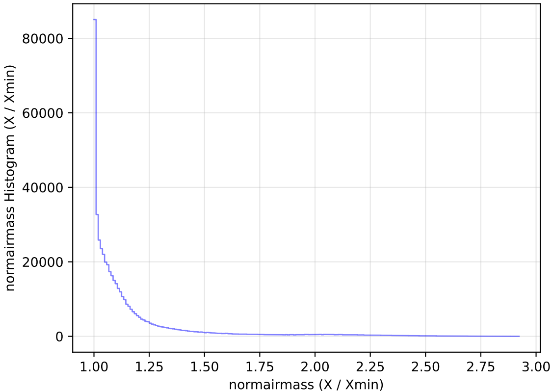
too_elab_r8_d3_gz_v3.4_10yrs All sky i band: normairmass Histogram
