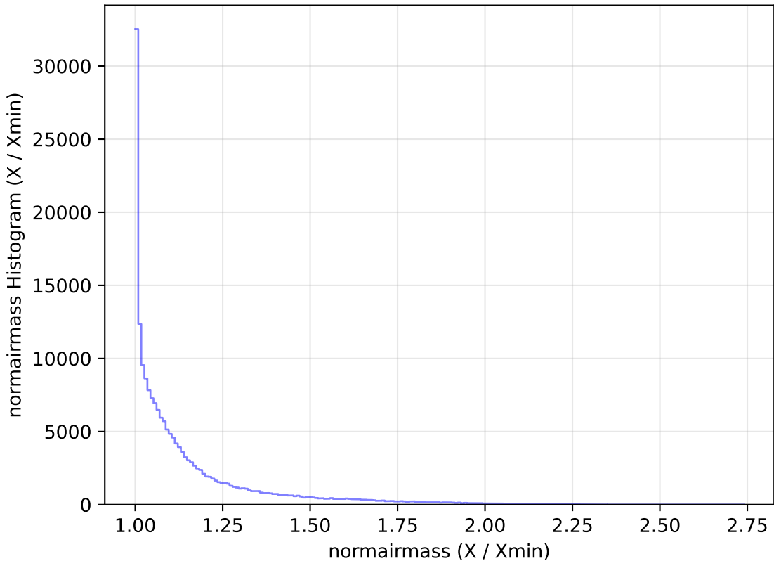
too_elab_r8_d3_gz_v3.4_10yrs All sky g band: normairmass Histogram
