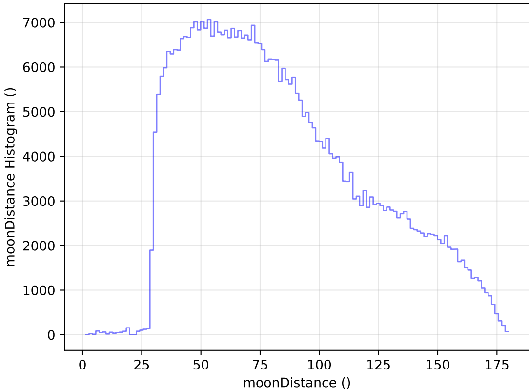
too_elab_r8_d3_gz_v3.4_10yrs WFD z band: moonDistance Histogram
