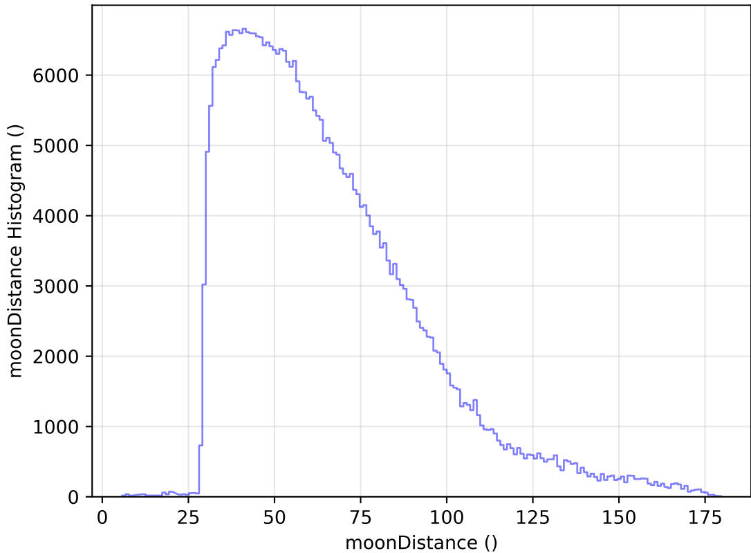
too_elab_r8_d3_gz_v3.4_10yrs WFD y band: moonDistance Histogram
