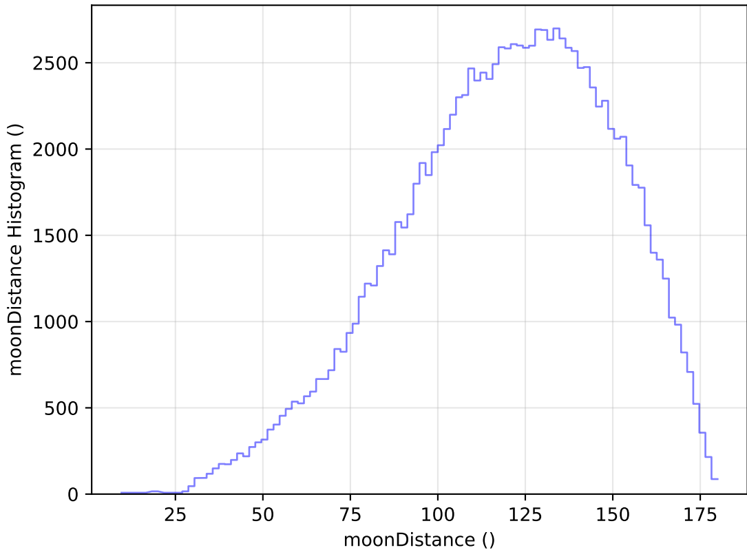
too_elab_r8_d3_gz_v3.4_10yrs WFD u band: moonDistance Histogram
